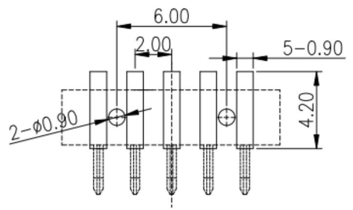
RECOMMENDED P.C.B LAYOUT TOP VIEW (.XX±0.05)
